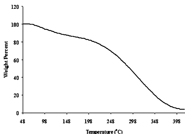
Figure 5. Thermogram of the cobalt-salen complex supported on activated carbon.
