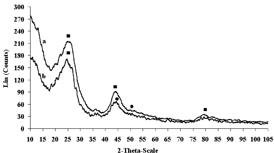
Figure 4. XRD patterns of activated carbon (a) and the cobalt-salen complex coated on activated carbon (b), amorphous carbon (■), Co (●).
