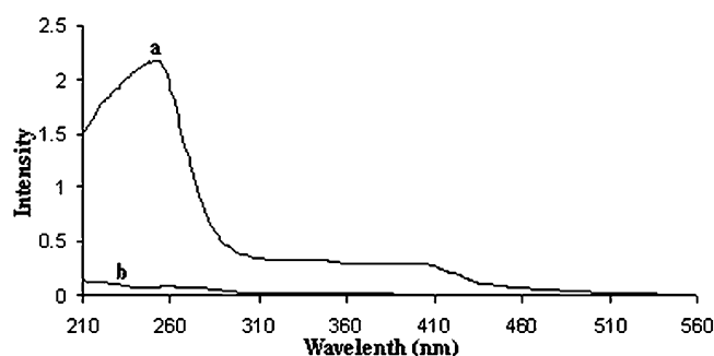
Scheme 2. Monitoring the supporting process of cobalt salen by the UV-Vis, (a): before and (b): after being supported on activated carbon.
