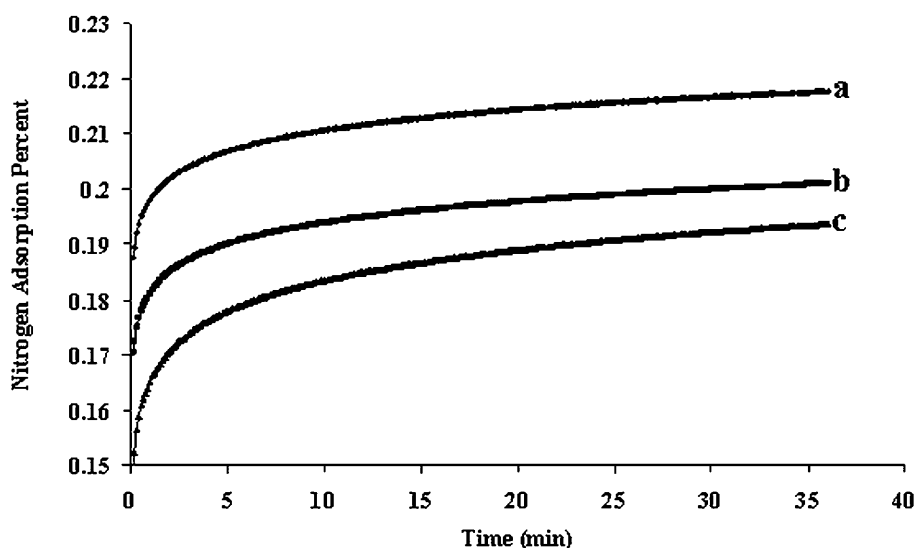
Figure 6. Comparison between the adsorption behaviour of nitrogen gas on carbon powder (a), carbon powder activated with oxygen (b) and activated carbon after deposition of the cobalt-salen complex (c).
