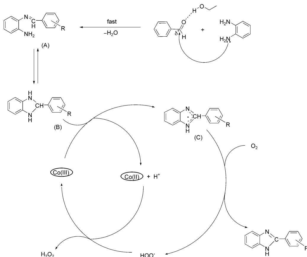
Scheme 4. The proposed mechanism for the cobalt-salen complex-catalyzed reaction for the synthesis of 2-substituted benzimidazole derivatives.
