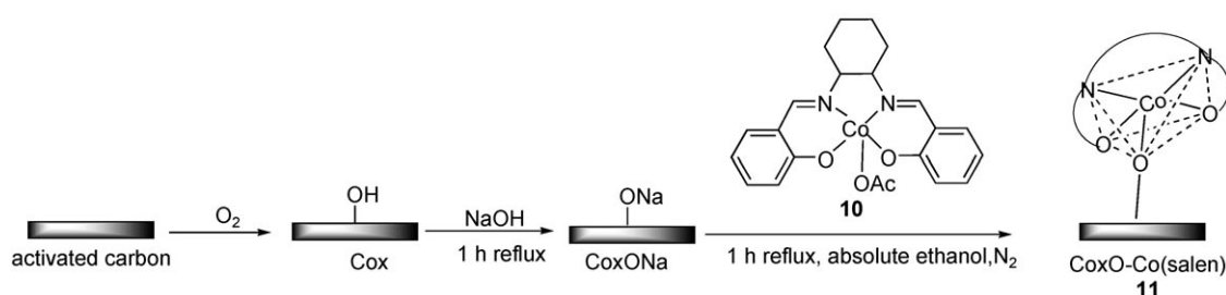
Scheme 3. The proposed anchoring procedure for the Co(salen) catalyst onto a modified air-oxidized activated carbon.
